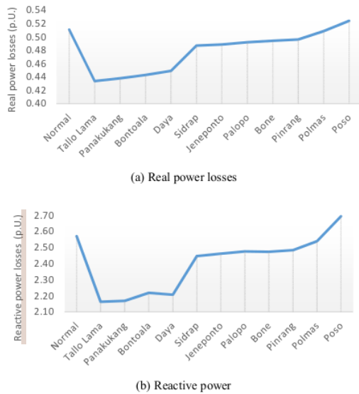
Fig. 8. Network Power Losses
