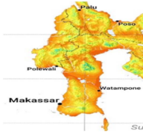
Fig. 4. Solar irradiance at Southern Sulawesi region
