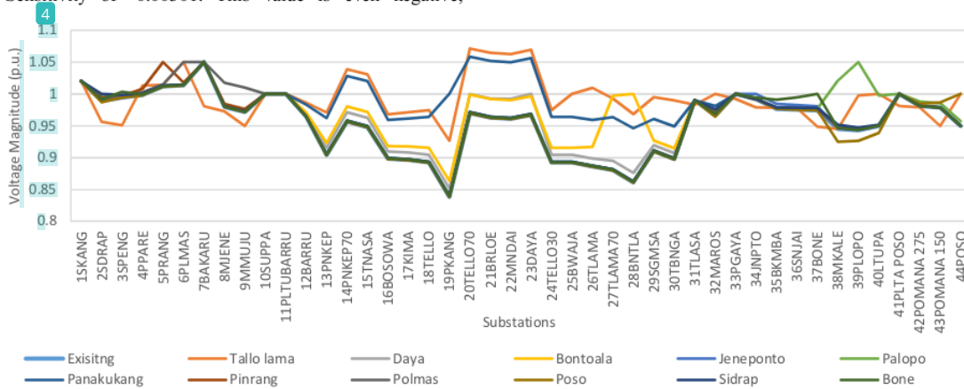
Fig. 6. Voltage Profiles for all scenarios
